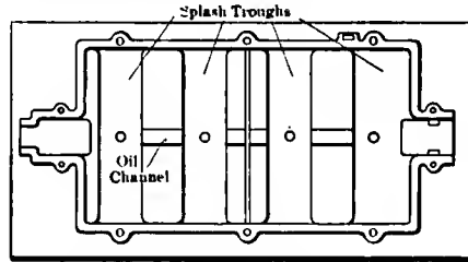
Fig. 2—Looking down into the oil reservoir as it is used on Kissal Kars
